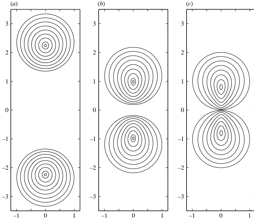
FIGURE 5. Pore closure, driven purely by surface tension, for pores at different initial separations: (a) \rho(0)=0.05 , (b) 0.3 and (c) 0.75. Here \beta=0 . The pores are shown at intervals of 0.25 with the final times shown in the figures ((a) to (c)) being t = 1.95, 1.88 and 1.75 . Note the elongation of the pores in the vertical direction and the downward motion of the pore centroids.
